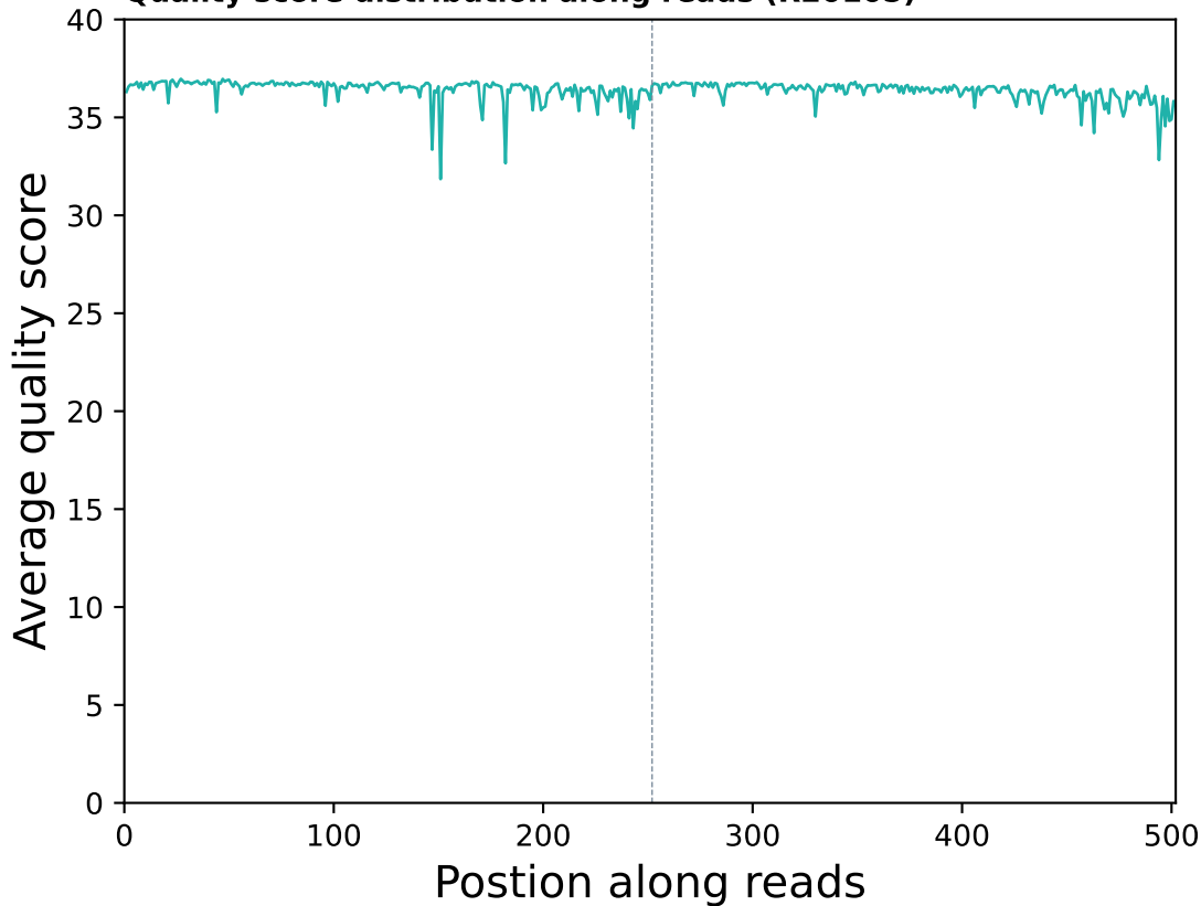
Quality score distribution along reads (R20105)
